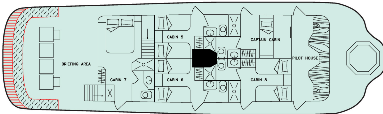
LEVEL THREE
